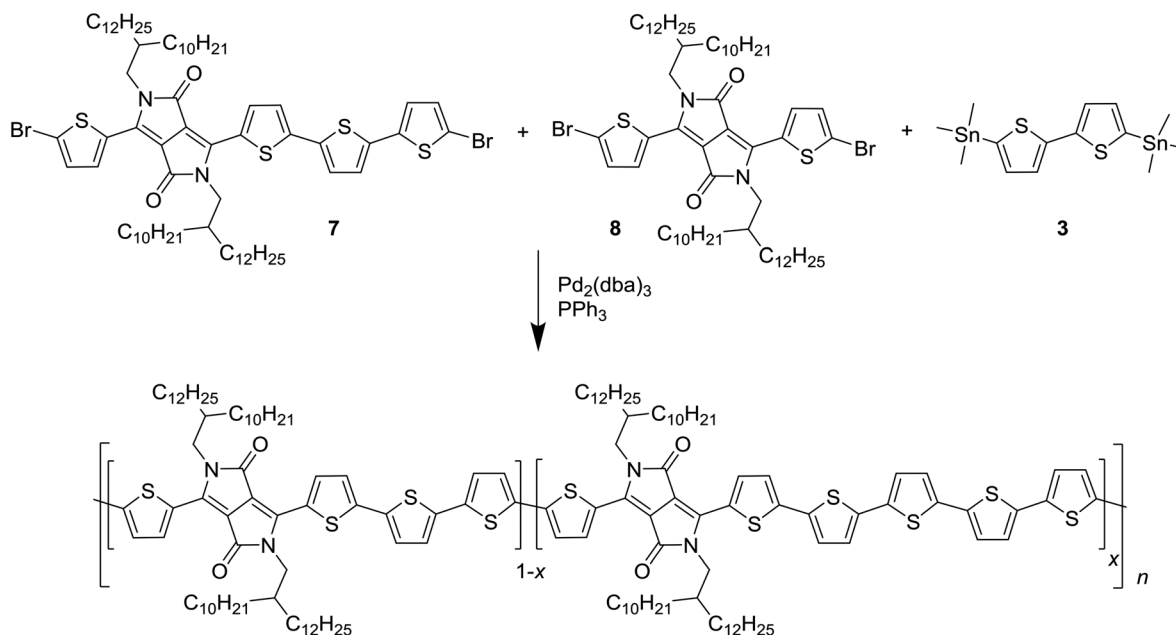
Scheme 3 Synthesis of the PDPP4T polymers with 6T defects. The stoichiometry of the monomers 7 and 8 was altered to obtain x = 0, 2, \text{ and } 5\% of intentional defects.
