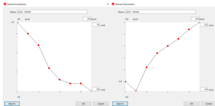
Figure 5. Implemented acceleration ( left )—deceleration ( right ) distributions for cyclists.
