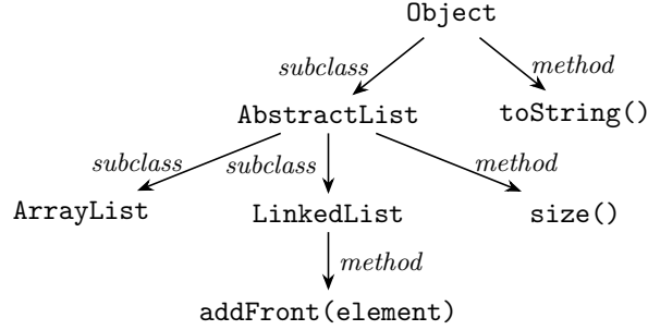
Figure 1: The hierarchical relations within typical list-classes in a Java-like object-oriented programming language.
