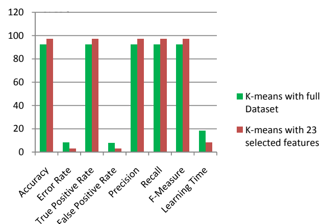
Fig. 3 Comparison chart between two K-means clustering methods
