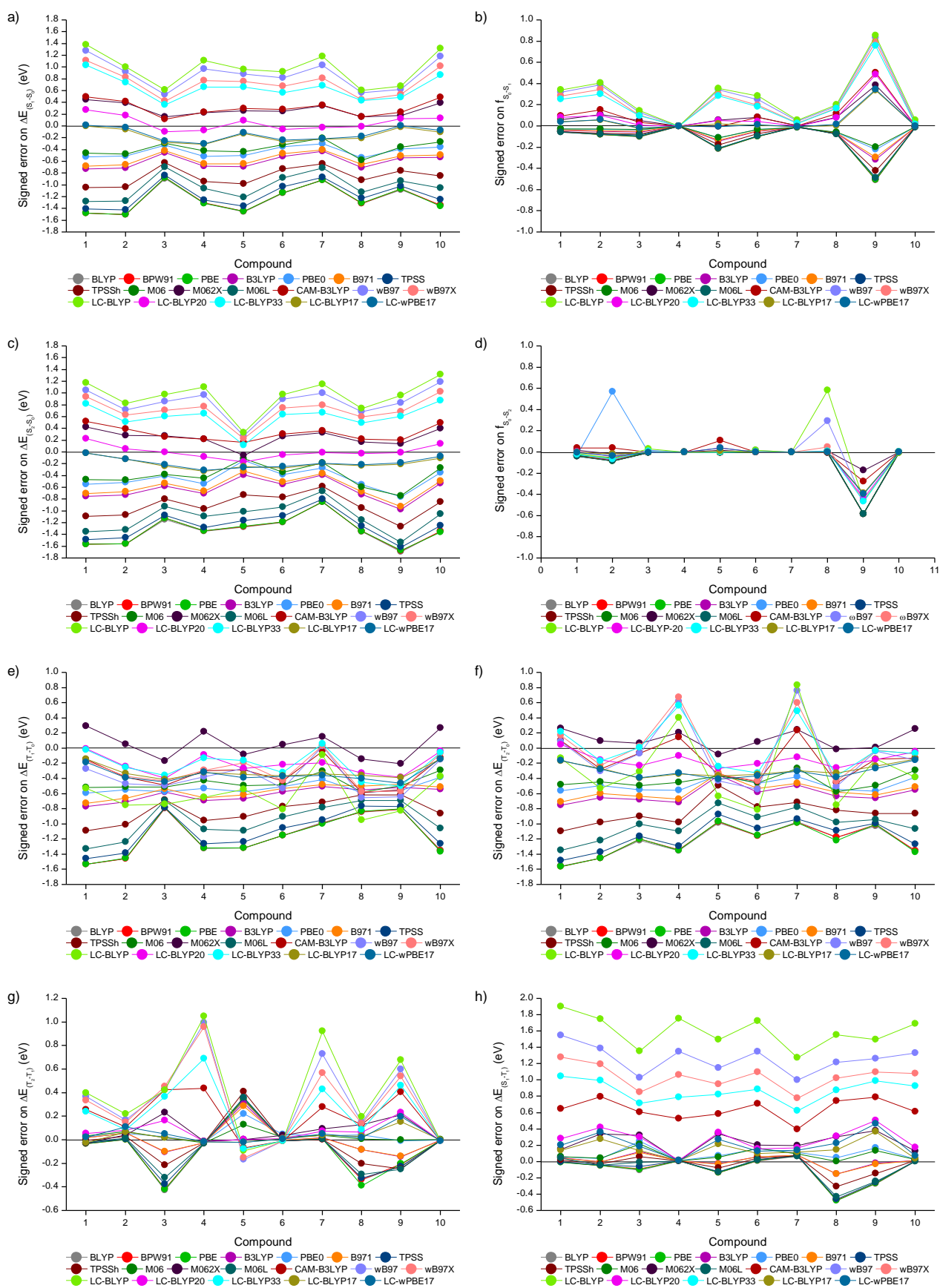
Fig. 3. Signed errors on each property for each individual XC functional for all 10 compounds obtained using TD-DFT. a) First vertical singlet excitation energy, \Delta E_{S_0 \rightarrow S_1} . b) Oscillator strength for the first singlet excitation, f_{S_0 \rightarrow S_1} . c) Second vertical singlet excitation energy, \Delta E_{S_2 \rightarrow S_0} . d) Oscillator strength for the second vertical singlet excitation, f_{S_2 \rightarrow S_0} . e) First vertical triplet excitation energy, \Delta E_{T_1 \rightarrow S_0} . f) Second vertical triplet excitation energy, \Delta E_{T_2 \rightarrow S_0} . g) Triplet-triplet energy gap for the first two triplet excited states, \Delta E_{T_2 \rightarrow T_1} . h) Singlet-triplet gap for the first singlet and triplet excited states, \Delta E_{S_1 \rightarrow T_1} .
