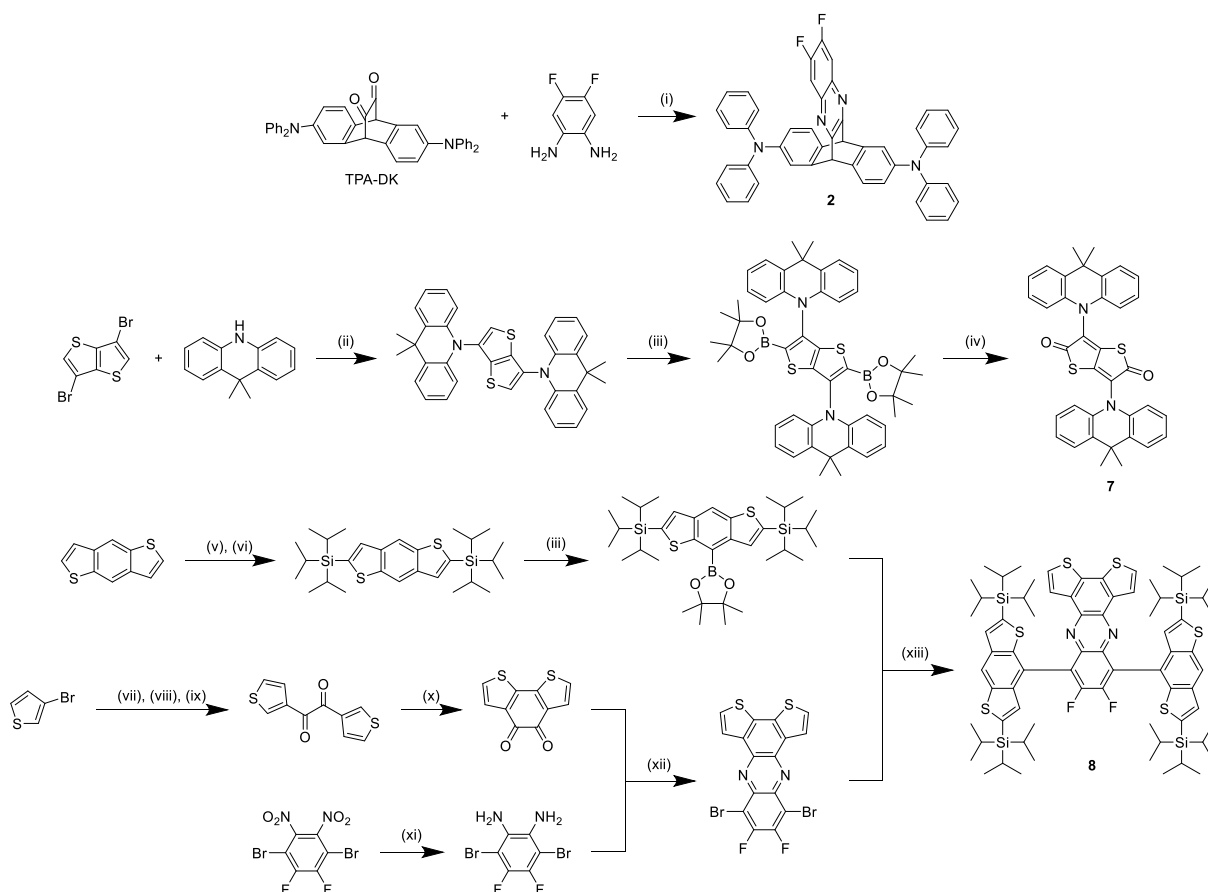
Scheme 1. Synthesis procedures for compounds 2 , 7 , and 8 : (i) ethanol/acetic acid (19/1) at reflux for 1 h; (ii) Pd(OAc) 2 , XPhos and Na(OtBu) in toluene at 110 °C for 24 h; (iii) bis(pinacolato)diboron, [Ir(OMe)(COD)] 2 , 4,4'-di- tert -butyl-2,2'-bipyridine in dry cyclohexane at 80 °C for 24 h; (iv) Oxone™ in THF/H 2 O (10/1) at room temperature for 3 h; (v) n -BuLi, dry THF at 0 °C for 1 h, (vi) TIPSCl, dry THF at 65 °C for 16 h; (vii) n -BuLi, dry THF at -78 °C for 1 h; (viii) CuBr, LiBr in dry THF at 0 °C for 1 h; (ix) oxalyl chloride at 0 °C for 1 h; (x) FeCl 3 , CH 3 NO 2 in CH 2 Cl 2 at room temperature for 3 h; (xi) iron powder in acetic acid at 45 °C for 6 h; (xii) acetic acid at 75 °C for 16 h; (xiii) Pd(PPh 3 ) 4 , K 2 CO 3 in DMF/H 2 O (4/1) at 130 °C for 24 h.
