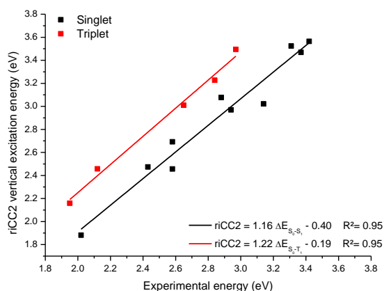
Fig. 2. Correlation plots between the riCC2 vertical excitation energies and the experimental values for maximum absorption \Delta E_{S_0-S_1} and \Delta E_{S_0-T_1} .
