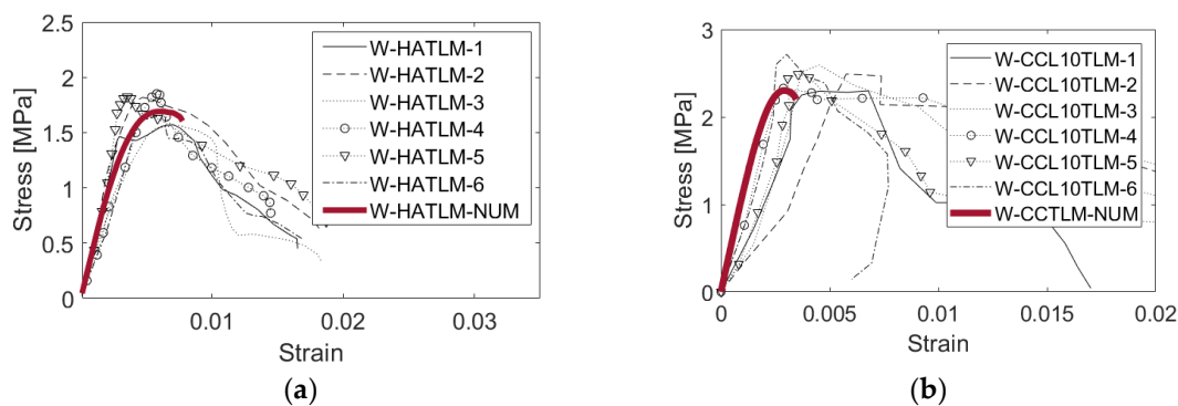
Figure 7. Numerical (in red color) and experimental (in black color) average stress-strain curves of: (a) homogeneous AAC masonry wallets; (b) composite AAC–clay wallets under centric compression.
