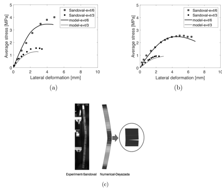
Figure 11. Validation of the model using Sandoval's experimental tests [18]: (a) effective average stress-lateral deformation curve with a slenderness of 18.7; (b) effective average stress-lateral deformation curve with a slenderness of 25.6; (c) failure pattern.
