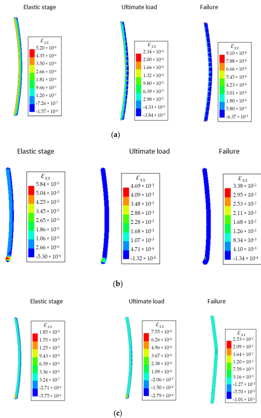
Figure 14. Horizontal normal strain contours for walls under pinned-pinned conditions at the elastic, ultimate load and failure stage under different amplitudes of load eccentricities and slenderness: (a) homogeneous clay wall with eccentricity e = t/3 and slenderness ratio h_{ef}/t = 26 ; (b) composite wall with eccentricity e = 0 and slenderness ratio h_{ef}/t = 21 ; (c) composite wall with eccentricity e = t/3 and slenderness ratio h_{ef}/t = 26 .
