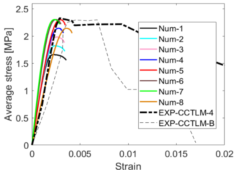
Figure 6. Obtained stress-strain curves throughout the numerical calibration process of a composite AAC–clay wallet model under centric compression.
