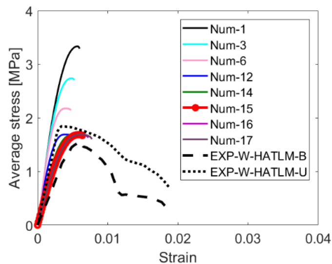
Figure 5. Obtained stress-strain curves throughout the numerical calibration process of a homogeneous AAC wallet model under centric compression.
