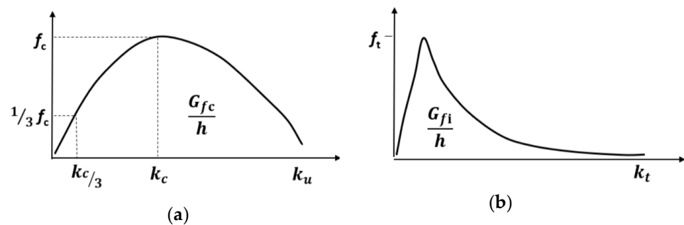
Figure 3. Stress-strain law adopted for: (a) uniaxial compression; (b) uniaxial tension.
