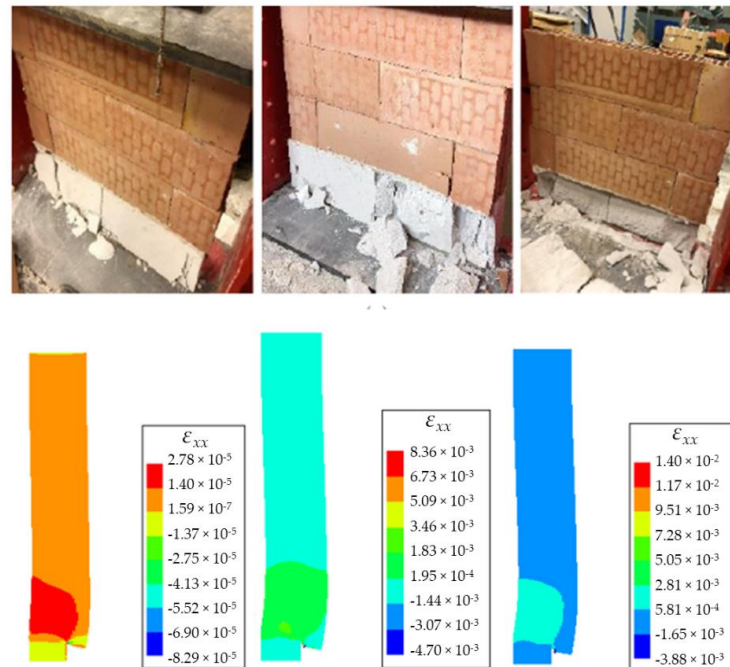
Figure 10. Numerical strain contours vs. experimental results [11] of the composite specimens in terms of failure behavior at the elastic stage (on the left side), ultimate load (in the center) and after failure (on the right side). For the numerical results, the contours of the horizontal normal strain are shown. Note that each subfigure has a separate color bar.
