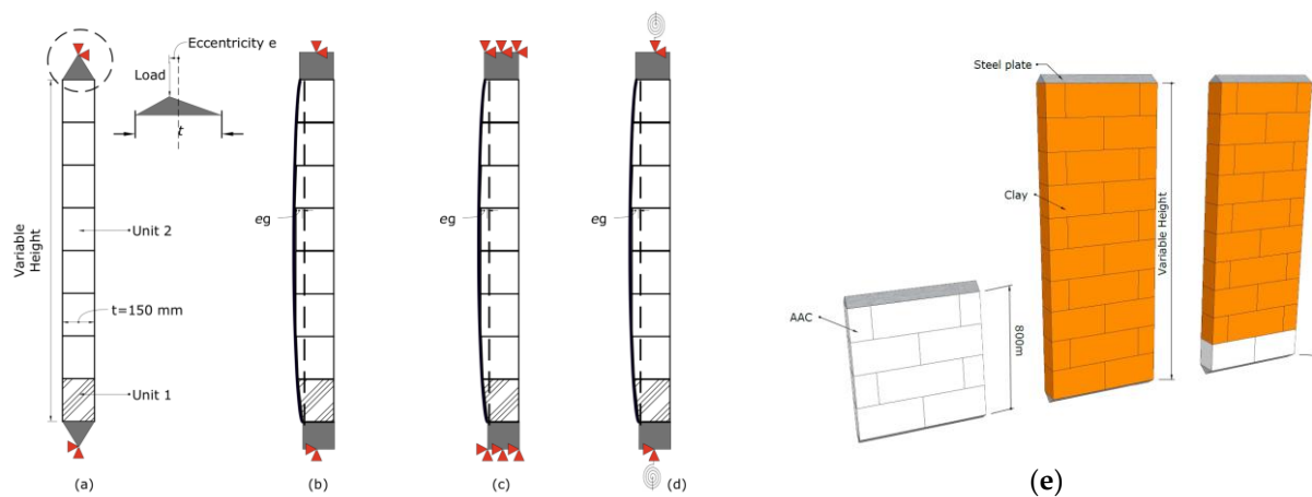
Figure 12. Model configurations for homogeneous and composite walls: (a,b) pinned-pinned conditions; (c) fixed-fixed conditions; (d) partially fixed-partially fixed conditions ( t is the wall thickness, e refers to the eccentricity of the load and e_g refers to the geometrical imperfection); (e) 3D configuration of homogeneous AAC, homogeneous clay and composite AAC–clay walls.
