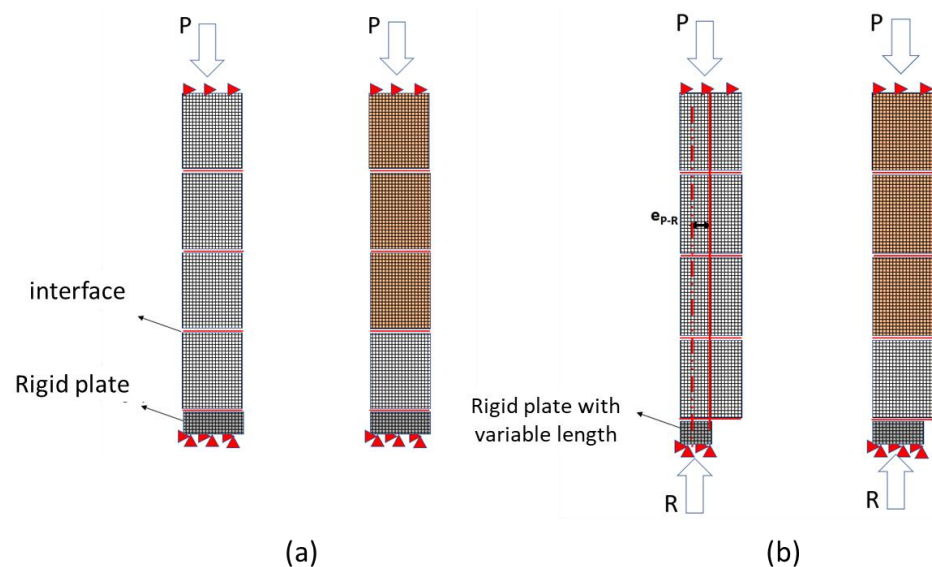
Figure 2. Model configuration of the tests on wallets: (a) centric compression; (b) eccentric compression with eccentricity e_{P-R} .
