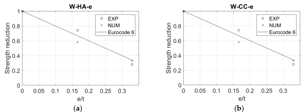
Figure 8. Numerical (a) vs. experimental (b) results in terms of strength reduction due to eccentricity.
