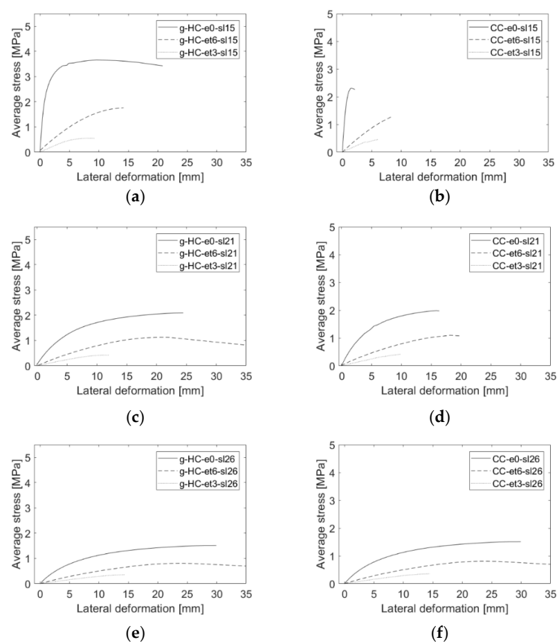
Figure 13. Average stress-lateral deformation curves for homogeneous (“H”) and composite (“C”) walls under different amplitudes of load eccentricities and slenderness: (a) homogeneous clay wall specimens with slenderness ratio (“sl”) h_{ef}/t = 15 ; (b) composite wall specimens with slenderness ratio h_{ef}/t = 15 ; (c) homogeneous clay wall specimens with slenderness ratio h_{ef}/t = 21 ; (d) composite wall specimens with slenderness ratio h_{ef}/t = 21 ; (e) homogeneous clay wall specimens with slenderness ratio h_{ef}/t = 26 ; (f) composite wall specimens with slenderness ratio h_{ef}/t = 26 . “e” refers to the amplitude of eccentricity.
