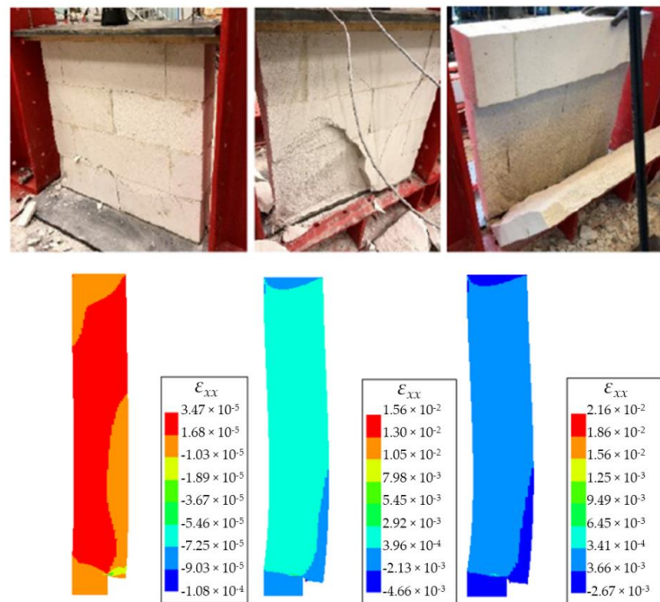
Figure 9. Numerical vs. experimental results of the homogeneous specimens in terms of failure behavior at elastic stage (on the left side), ultimate load (in the center) and after failure (on the right side). For the numerical results, the contours of the horizontal normal strain are shown. Note that each subfigure has a separate color bar.
