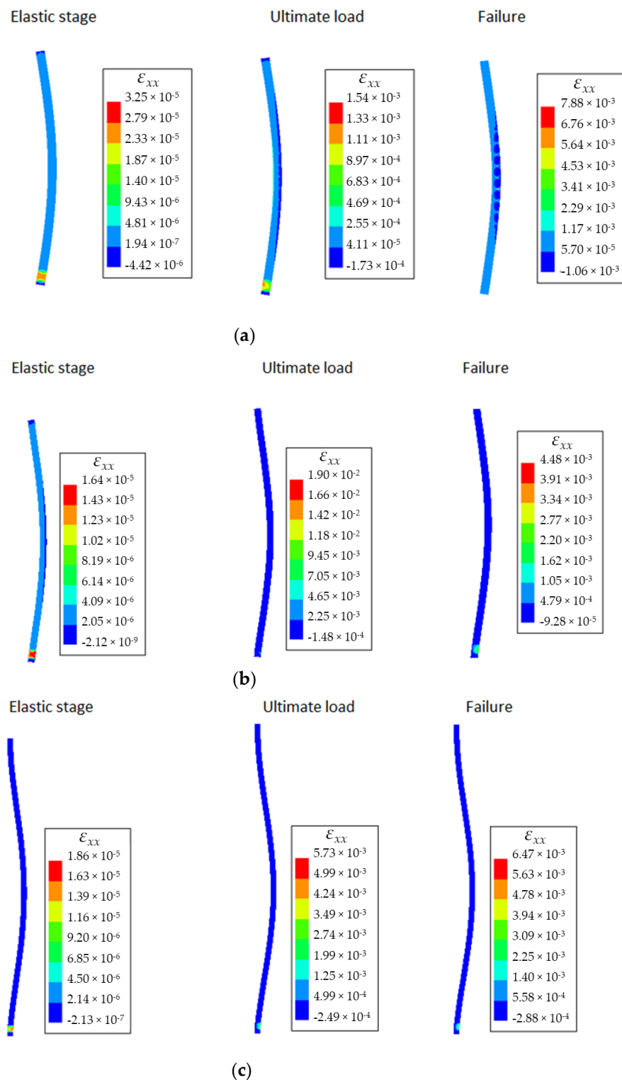
Figure 15. Horizontal normal strain contours for walls under different boundary conditions at the elastic, ultimate load and failure stage (eccentricity e = 0 and slenderness ratio 26): (a) composite wall under pinned-pinned conditions; (b) composite wall under partially fixed-partially fixed conditions; (c) composite wall under fixed-fixed conditions.
