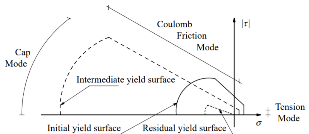
Figure 4. The rate-independent interface model. Adapted from Lourenço (1996) [36].
