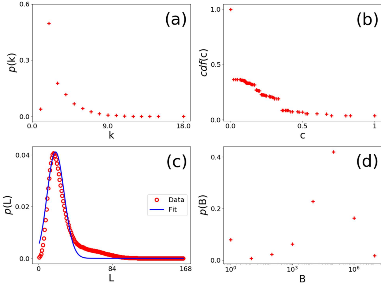
Fig. 1. Topological characteristics of the Beijing bus-subway coupled network. (a) probability distribution of degrees, (b) cumulative distribution of cluster coefficient, (c) probability distribution of shortest path length, (d) probability distribution of betweenness (log-binning).
