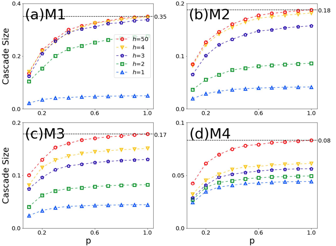
Fig. 2. Relative cascading failure size as a function of initial failure nodes.
