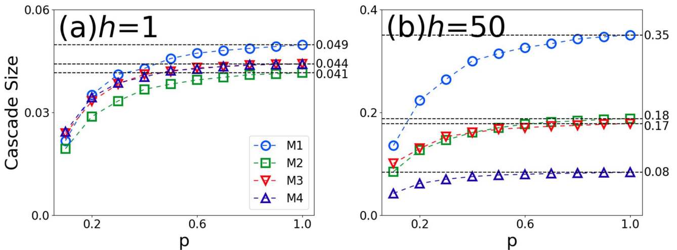
Fig. 3. Relative cascading failure size as a function of initial failure nodes.
