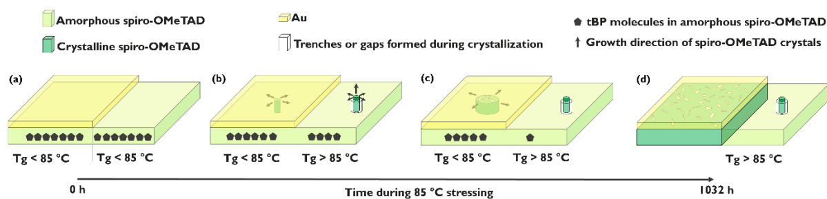
Figure 3. (a-d) Schematics showing the hypothesis of the mechanism of spiro-OMeTAD film morphology evolution in PSCs during 1032-hour 85 °C thermal stressing.
