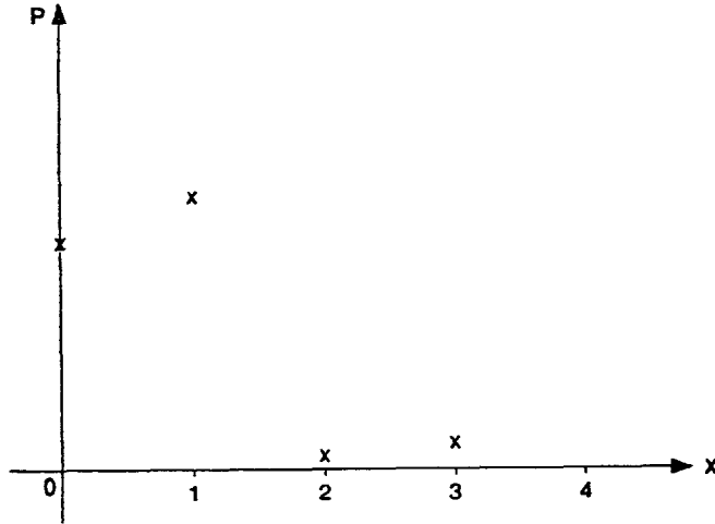
Figure 3. Partial graph of p .
