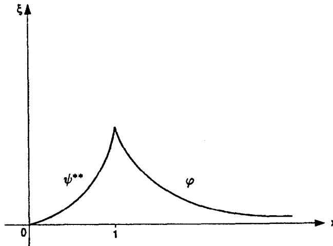
Figure 1. Lotka's law and its dual: primitive model of the fraction of the authors with x papers.
