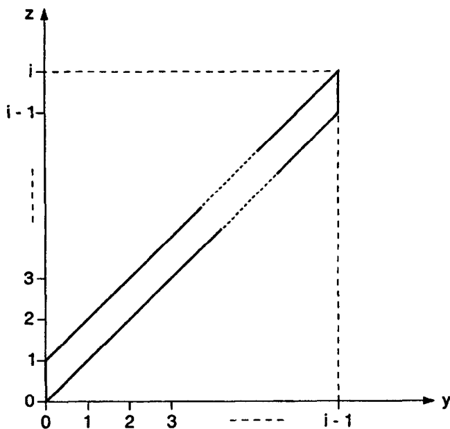
Figure 2. Integration domain for f_i , for every z, i = 2, 3, \dots
