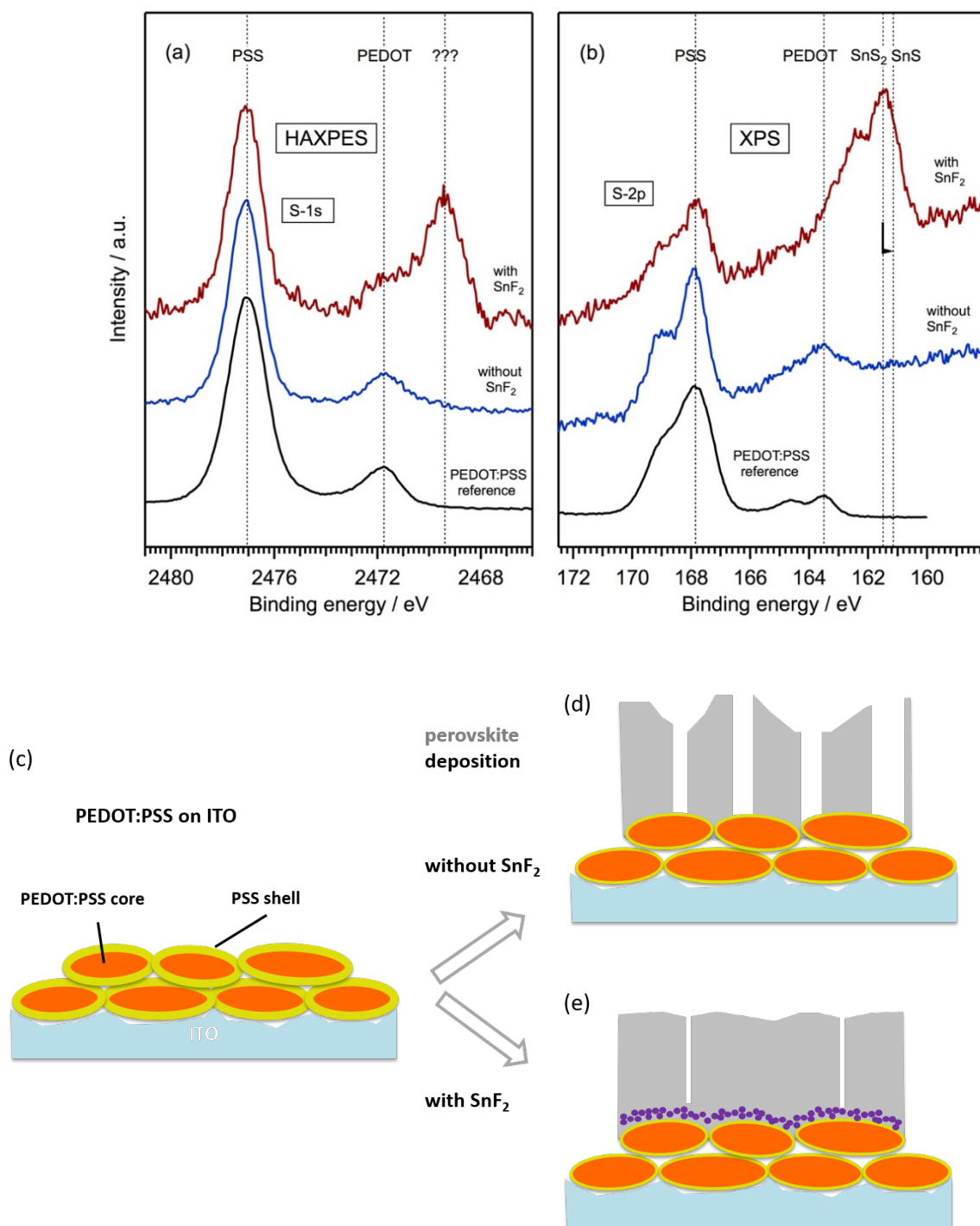
Figure 3. HAXPES results for the S-1s core level region (a) and XPS results for the S-2p binding energy range (b) measured on samples without (blue curves) and with (red curves) SnF 2 additive. Related core level spectra acquired on a pure PEDOT:PSS film have been added as reference. Binding energy values taken from literature [32] for SnS as well as SnS 2 have been added as vertical lines. Schematics (c-e) visualize the conclusions drawn from the experimental photoemission spectra of formed SnS nanoparticles/nanograins/nanoclusters in violet.
