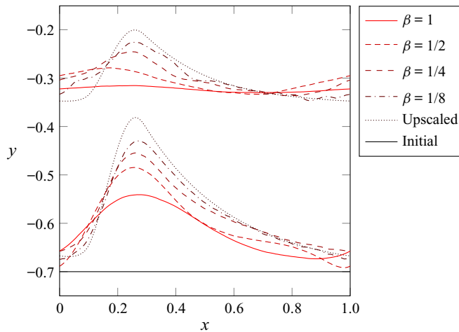
Figure 6. Interface locations at time t = 2.4 for the non-dimensional \delta -2f1s-model with varying \beta , and for the upscaled \delta -2f1s-model. The fluid–fluid interface can be seen in the upper half and is located by the condition \phi_1 = \phi_2 . The fluid–solid interface in the lower half is located by \phi_1 = \phi_3 . The initial location of the fluid–solid interface is marked by a black line.
