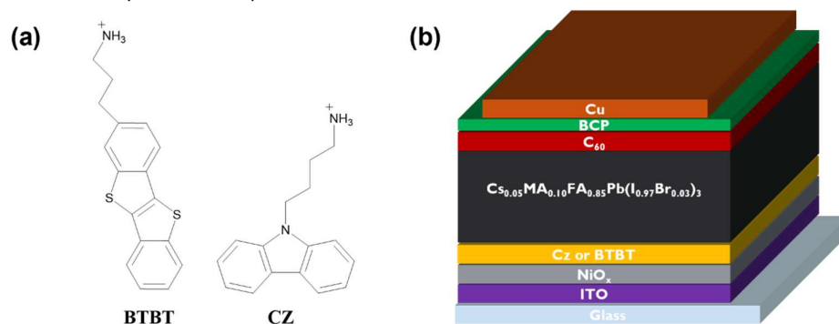
Fig. 1: (a) Molecular structure of BTBT and Cz. (b) Perovskite solar cell stack depiction. The control sample does not contain any modification between \text{NiO}_x and the perovskite layer.
