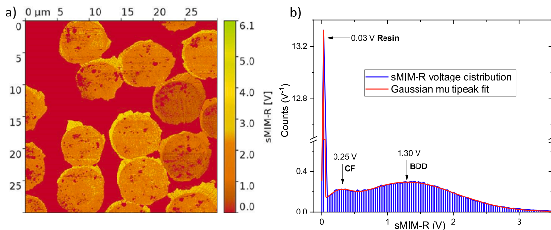
Fig. 6. sMIM cross-sectional measurement on BDD-CF upright standing position. a) sMIM-Resistive signal map scan in forward direction. b) sMIM-Resistive signal distribution of the same region.
