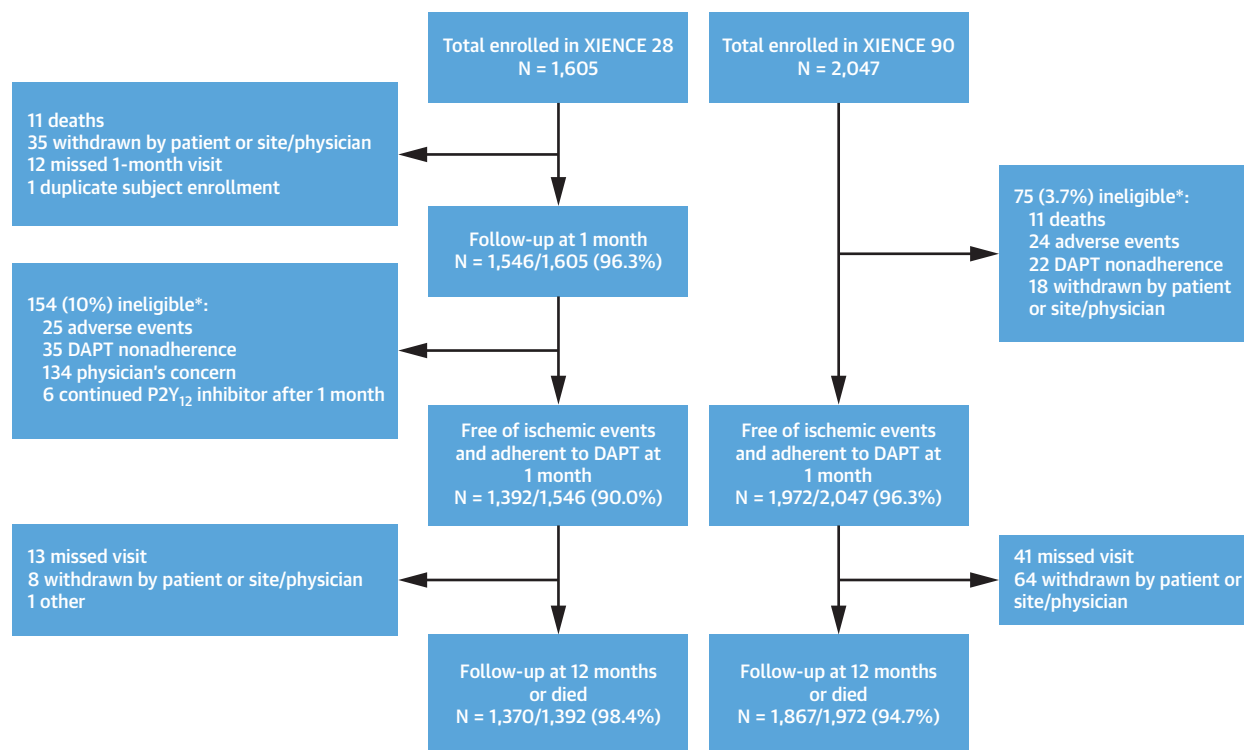
FIGURE 1 Study Flowchart
