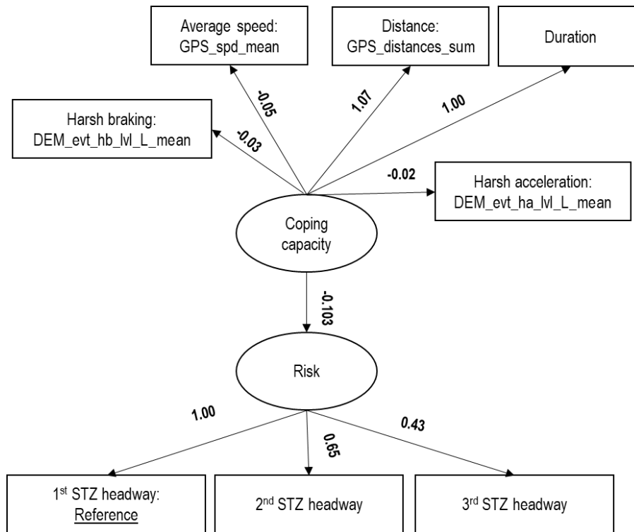
Figure 30: Results of SEM on Risk (Headway STZ) – Portuguese bus drivers – experiment Phase 2
