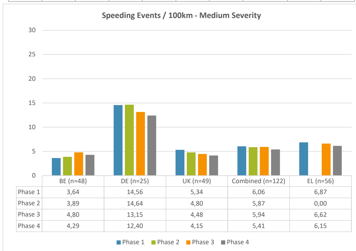
Figure 11: Medium speeding events / 100km per country and per phase (cars)
