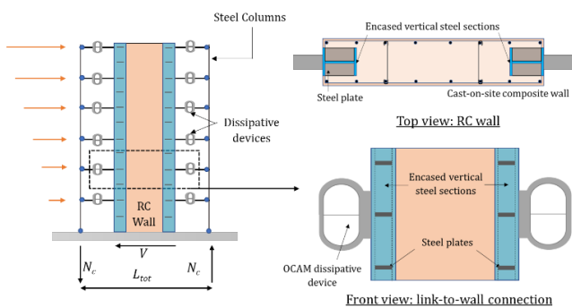
Figure 4 Schematic diagram of Configuration 3.
