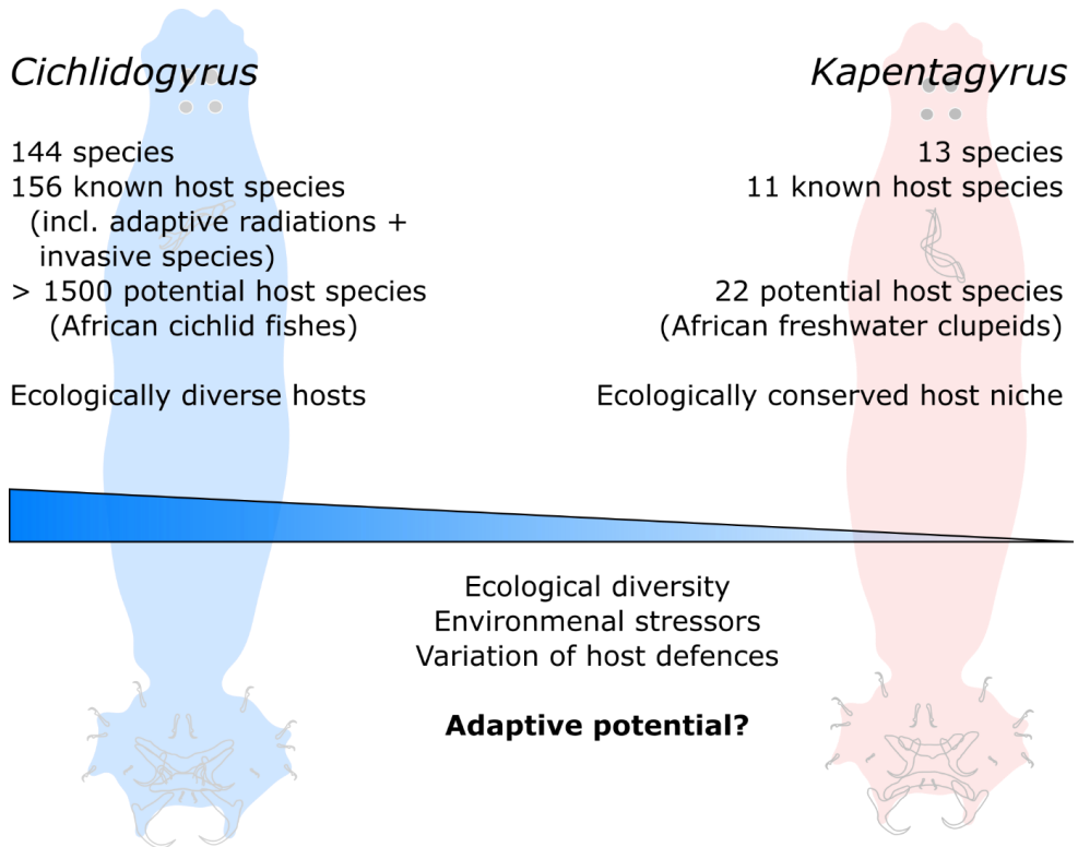
Figure 6.1. Overview of species richness and ecological diversity of species of two dactylogyrid monogenean genera: Cichlidogyrus and Kapentagyryrus .
