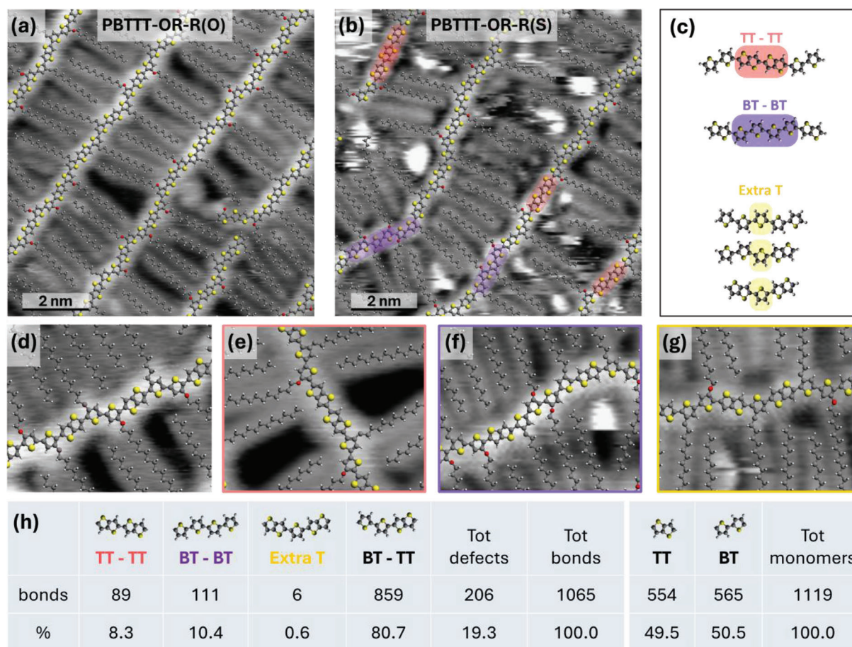
Figure 4. a) High-resolution STM image of self-assembled PBTTT-OR-R(O), and b) PBTTT-OR-R(S) with the corresponding molecular models superimposed. c) Types of polymerization defects considered for fitting the STM images: TT and BT homocoupling, and the three possible cases of sequences with a single extra T. Zoomed-in details displaying d) the expected, defect-free alternating BT-TT sequence, e) TT homocoupling, f) BT homocoupling, and g) extra T defect. h) Frequencies of polymerization defects and monomers observed in PBTTT-OR-R(S). The frequencies of the defects were normalized by the total number of bonds between TT and BT units, and the monomers frequencies by the total number of TT and BT units.
