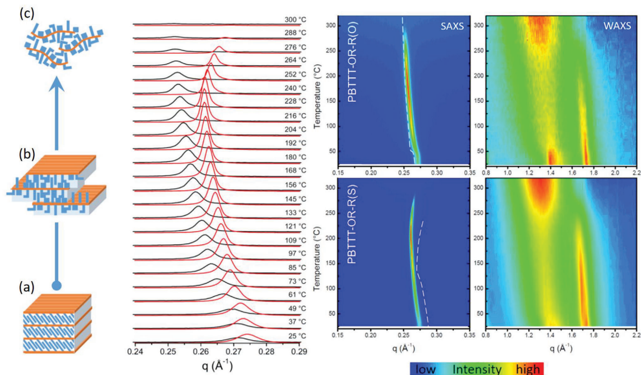
Figure 6. Selected temperature-resolved SAXS patterns of PBTTT-OR-R(O) (black) and PBTTT-OR-R(S) (red) and all top-view color-coded SAXS/WAXS data during heating at 50 \text{ K min}^{-1} after cooling at 20 \text{ K min}^{-1} for PBTTT(O) and after cooling at 5 \text{ K min}^{-1} for PBTTT(S) (top panels: SAXS and WAXS of PBTTT-OR-R(O); bottom panels: SAXS and WAXS of PBTTT-OR-R(S)). Left: Schematic representation of conversion from the crystalline a) to the sanidic liquid crystalline state b) by side chain (blue lines) melting, followed by backbone (orange lines) melting into the fully molten state c). The dashed white lines in the colored SAXS panels of PBTTT-OR-R(O) and PBTTT-OR-R(S) are from PBTTT-(OR) 2 (O) and PBTTT(S), respectively (for comparison). [17]
