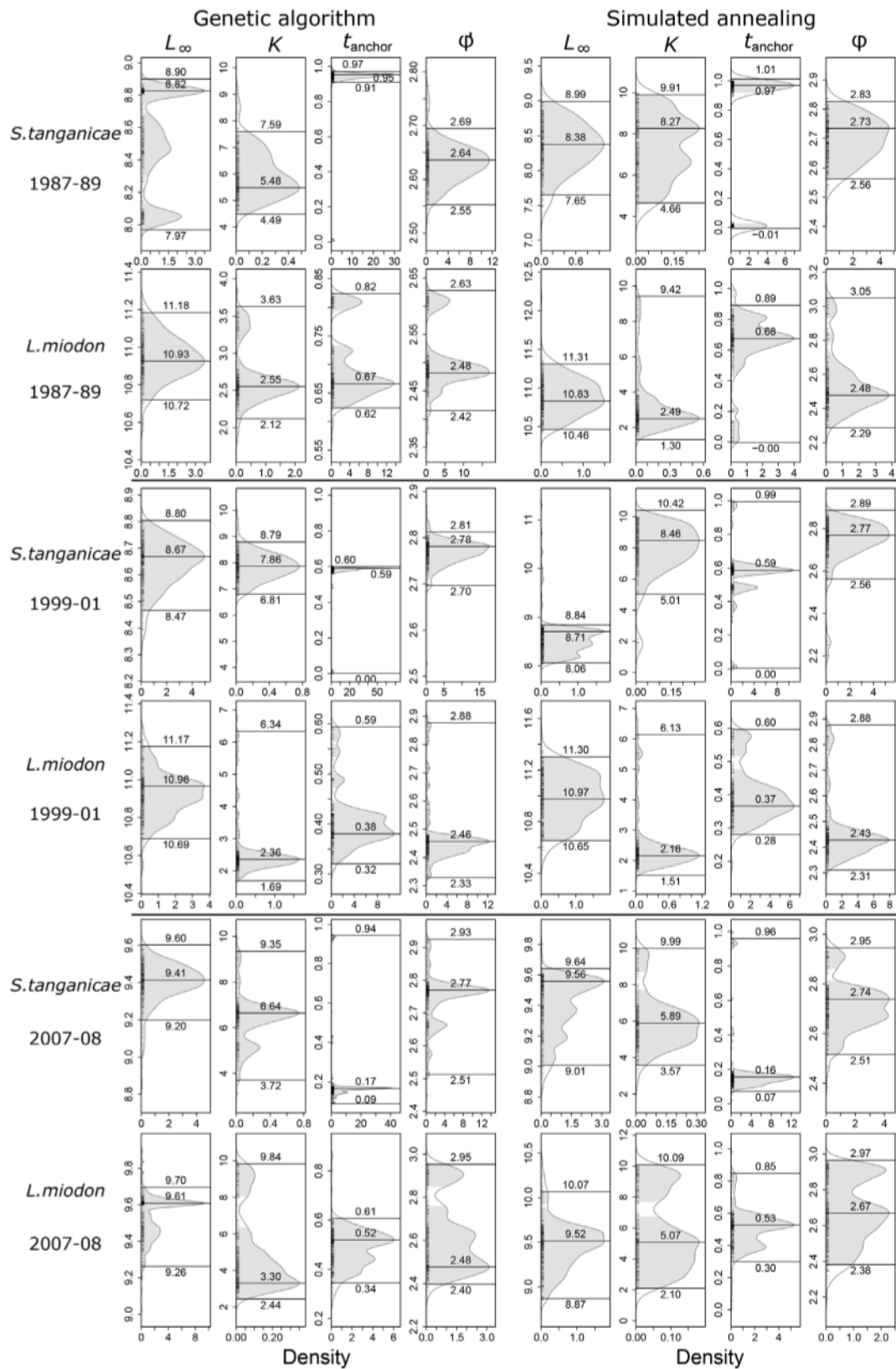
Supplementary figure 2 – Probability distribution of estimated parameters using genetic and simulated annealing algorithms for Stoltothrissa tanganicae and Limnothrissa miodon in each study period.
