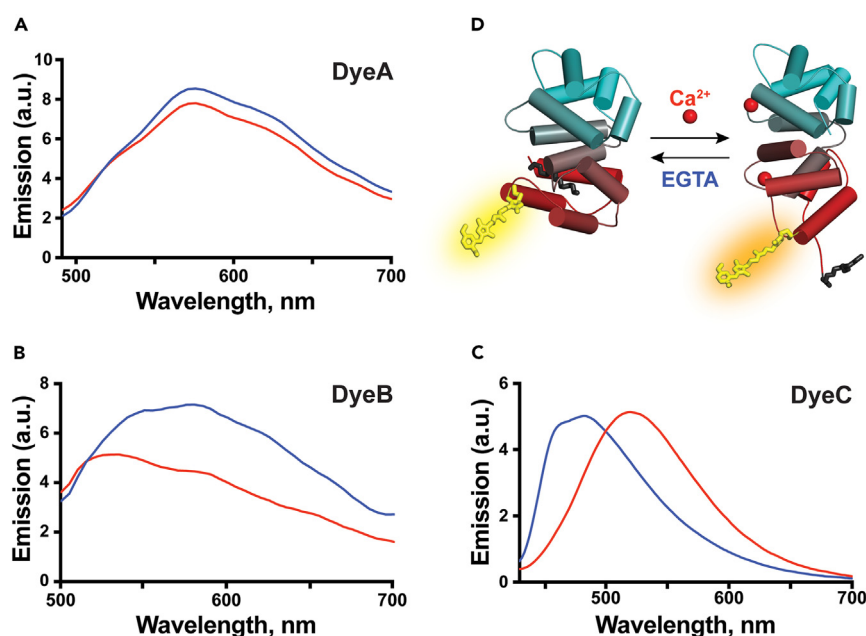
Figure 2. \text{Ca}^{2+} -induced conformational and spectral changes of Rec labeled with DyeA, DyeB, and DyeC
