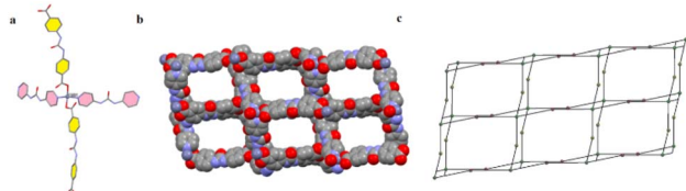
Fig. 2 (a) Representation of the coordination environment around \text{Zn}(\text{II}) for UA-1, (b) the space-filling model of the channel of UA-1 along the [010] direction (solvent removed) and (c) simplified view of the polycatenated array with dia; 4/6/c1; sqc6 topology for UA-1.
