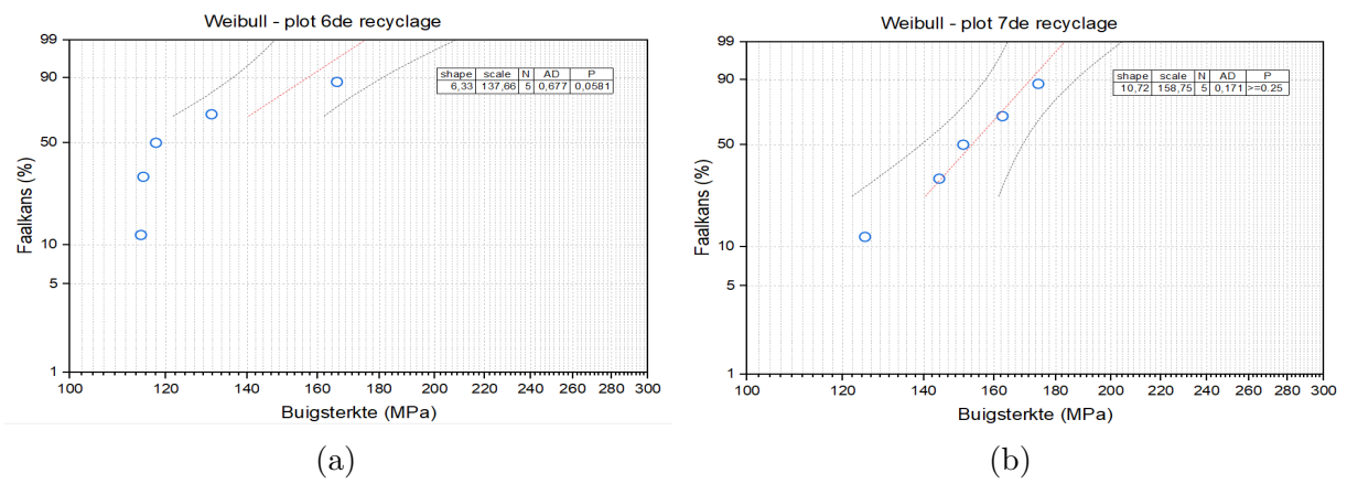
Figuur 5: (a) Weibull-plot 6de recyclage ; (b) Weibull-plot 7de recyclage feedstock
