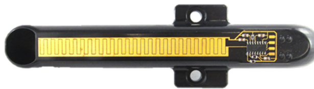
Figure 12. Dip pipe sensor with level detection electronic [109].
