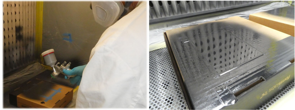
Figure 9. Processing of the MID lacquer using the HVLP technology.
