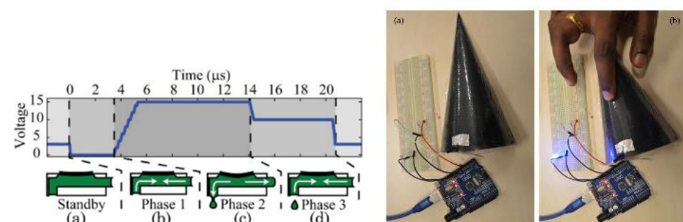
Figure 6. (Left): Voltage waveform for inkjet printing [45]. (Right): Capacitive touch sensor using inkjet printing and 3D forming [29].
