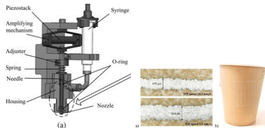
Figure 5. (left): Piezo-driven dispenser for valve-jet printing [42]. (Right): Printed line width for 50% and with a constant DL of 19 ms [43].
