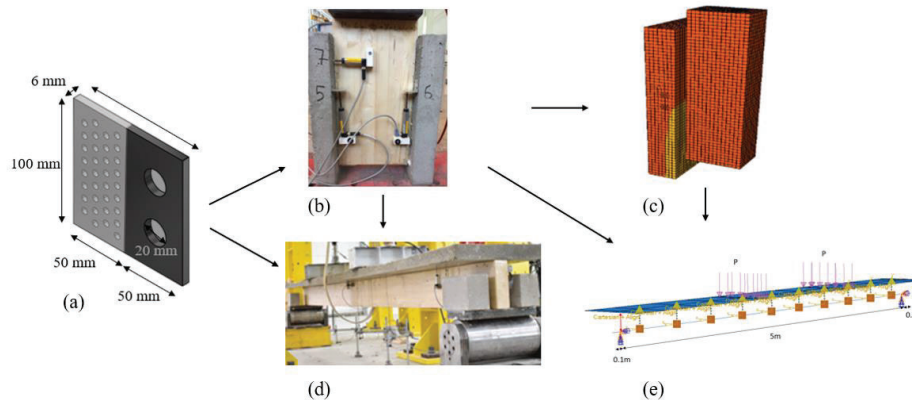
Figure 1: Test specimens: (a) PerFOBOND plate dimensions; (b) Shear test specimen; (c) shear test Abaqus model, (d) Bending test specimen and (e) bending test Abaqus model.
