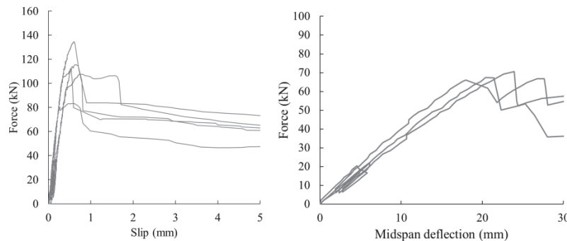
Figure 3: Experimental results, from left to right: (a) Force-slip curve of shear tests, P-ST; (b) Force-midspan deflection curve of bending tests, P-BT.
