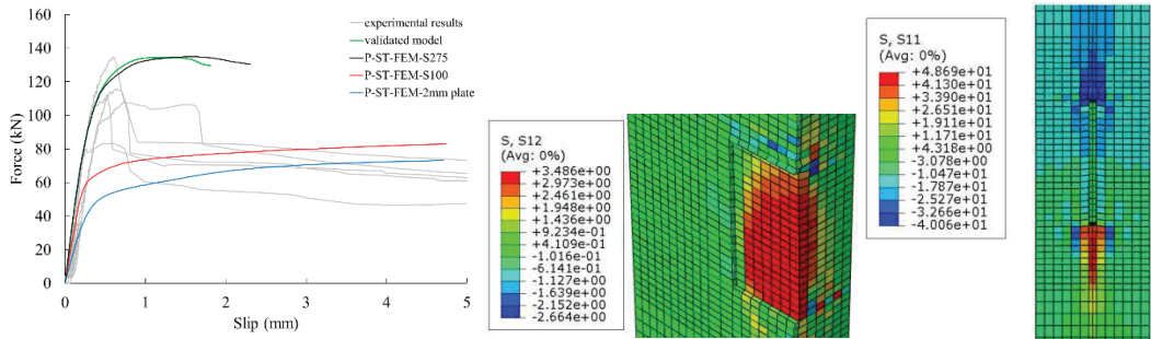
Figure 4: Numerical analysis results, from left to right: (a) Force-slip curve of the validated model against experiments and parametric study; (b) Shear distribution at the groove – the fibers reaching shear capacity; (c) Crushing of the timber under the perfobond plate.
