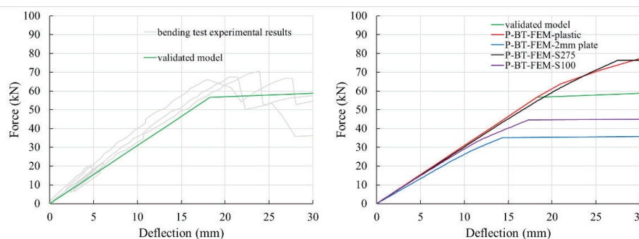
Figure 5: Force-midspan deflection curves, from left to right: (a) Experimental and validated model; (b) Parametric study.
