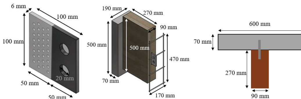
Figure 2: Test specimens, from left to right: (a) PerFOBOND plate dimensions; (b) Shear test specimen cross-section; (c) Cross-section of the TCC beam tested in bending.
