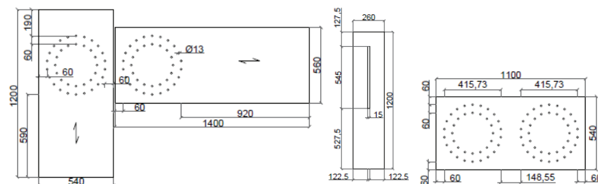
Figure 4: MR-2 specimen, from left to right: (a) Front view of column-beam joint; (b) Side view of the column; (c) Front view of the steel plate. All dimensions are in millimeters.
