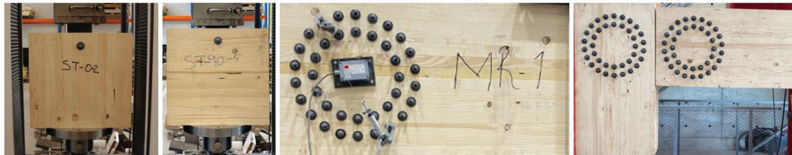
Figure 1: Test specimens, from left to right: (a) Shear test where the threaded rod is parallel to the grain, ST-0; (b) Shear test where the threaded rod is perpendicular to the grain, ST-90; (c) Single moment connection, MR-1; (d) Column-beam moment connection, MR-2.
