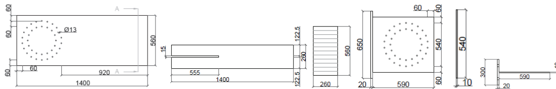
Figure 3: MR-1 specimen dimensions, from left to right: (a) Front view of the timber beam; (b) Top view of the timber beam; (c) Cross-section of the timber beam; (d) Front view of the steel plate; (e) Cross-section of the steel plate; (f) Top view of the steel plate. All dimensions are in millimeters.
