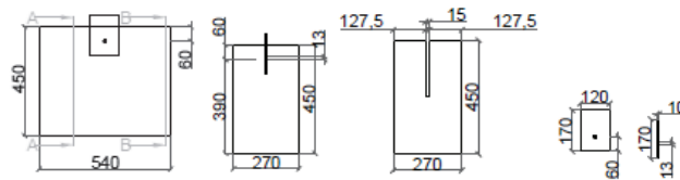
Figure 2: Specimen dimension of the shear tests (same for both ST-0 and ST90), from left to right: (a) Front view; (b) Cross-section A-A; (c) Cross-section B-B; (d) Front view of the steel plate; (e) Side view of the steel plate. All dimensions are in millimeters.
