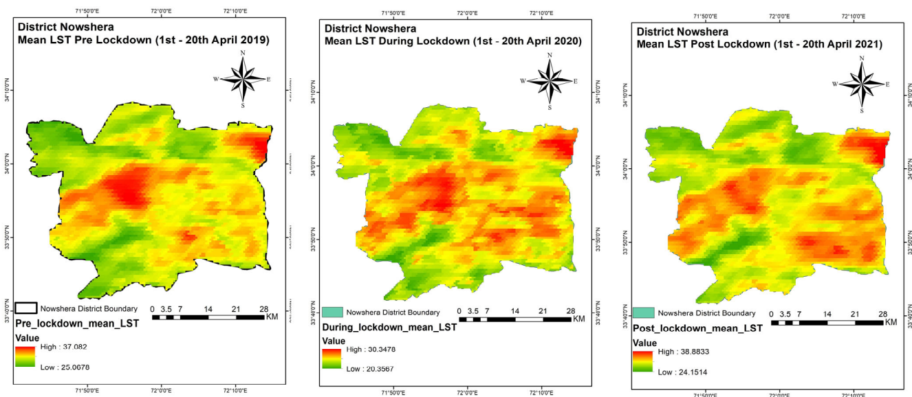
Figure 3. LST Trends Across Pre-, During-, and Post-Lockdown Phases in Nowshera District (April 2019–2021).
