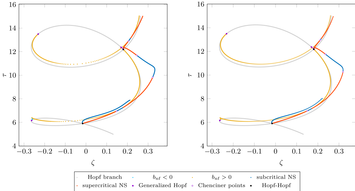
Figure 2: Bifurcation diagrams of (70) with unfolding parameters (\zeta, \tau) . The left figure is obtained via periodic normalization in DDEs while right figure is obtained via a pseudospectral approximation.
