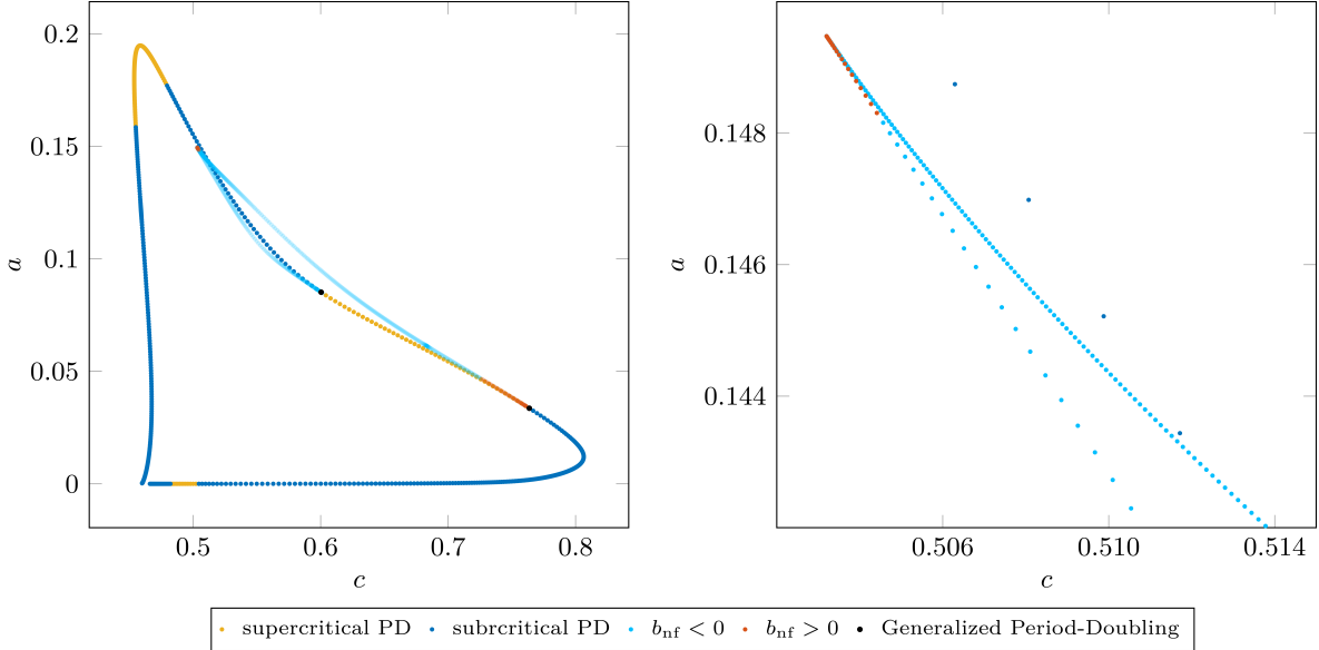
Figure 1: Bifurcation diagrams of (69) with unfolding parameters (a, c) . Left, sub- and supercritical period-doubling (PD) branches are shown, with two identified generalized period-doubling points connected by a limit point of cycles branch. Right, a close-up near the cusp bifurcation located on the LPC-branch.
