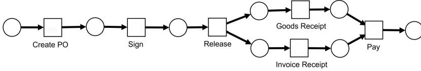
(a) Normative model for the purchase to pay process in Petri-net
