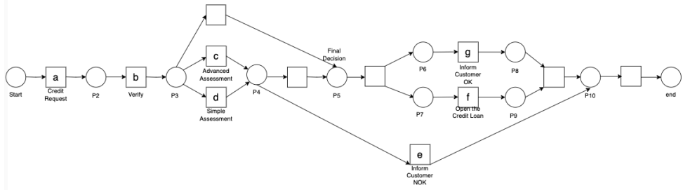
Figure 5.5: Petri Net model of the Credit Request model of Figure 5.3
