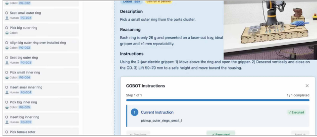
(b) Execution view with human instructions and cobot actions (Step 5).
