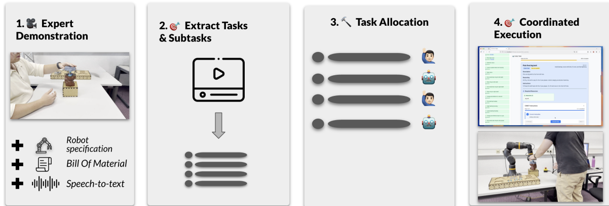
Figure 1: DELEGACT’s human-in-the-loop pipeline for task-level human–robot collaboration. (1) An expert performs a narrated manual assembly. (2) A vision–language model extracts structured steps and atomic subtasks grounded in video frames and transcript. (3) A language model proposes human–cobot task allocations based on robot specifications, operator competencies, and bill-of-material constraints. (4) An interactive interface supports inspection, editing, and coordinated execution with triggerable cobot actions.
