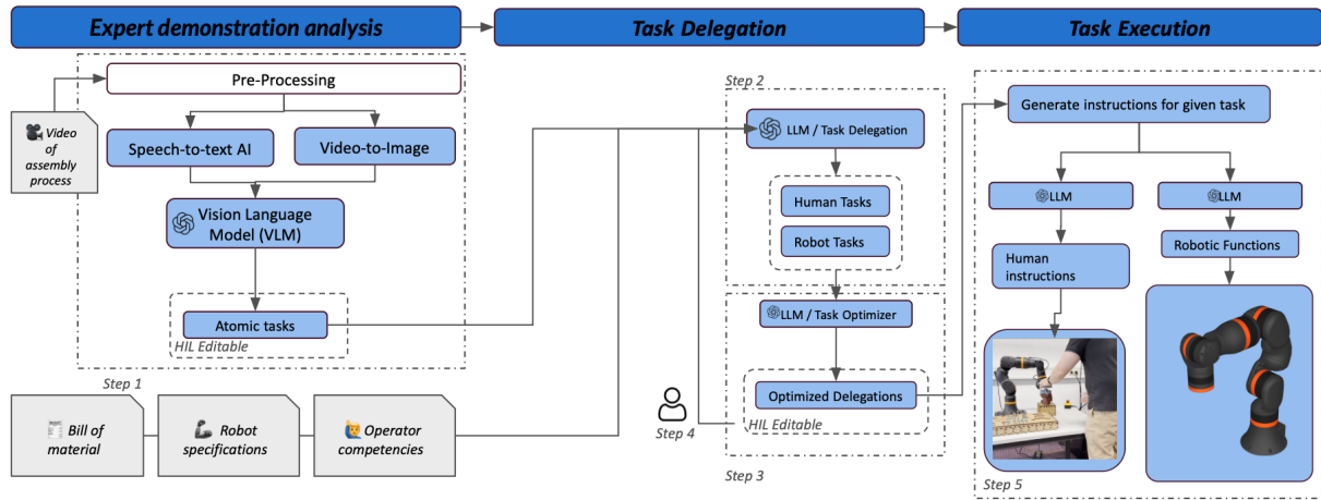
Figure 3: System architecture of DELEGACT. The pipeline consists of three stages: (1) Expert demonstration analysis with speech-to-text transcription and frame sampling for vision-language task extraction; (2) Task delegation using LLM-based human-cobot assignment and workflow optimization; (3) Task execution via parameterized robot behavior templates and generated human instructions.
