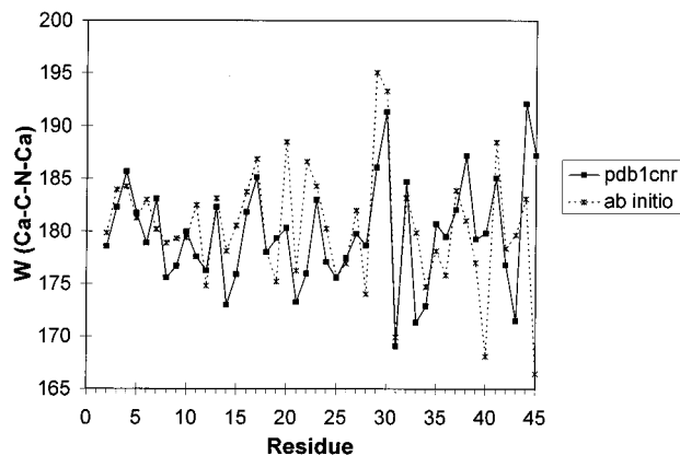
Figure 4. Comparison of crystallographic (pdb1cncr) 51 and HF/4-21G optimized \omega -torsional angles of crambin.
