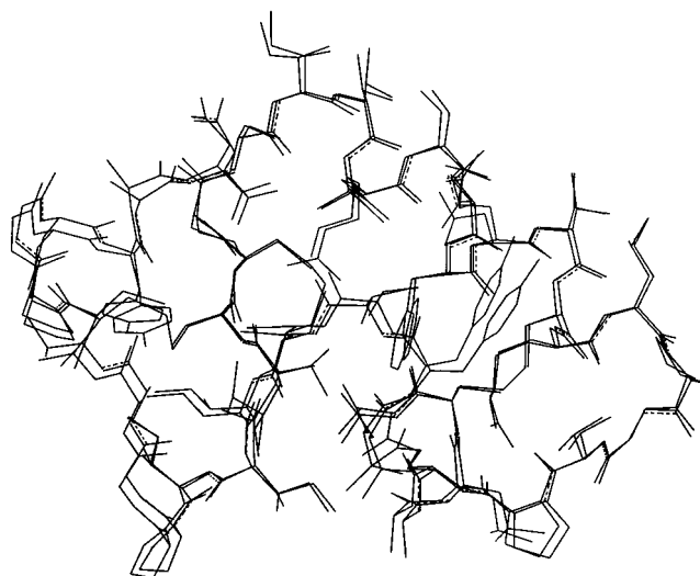
Figure 5. Superposition of the crystallographic (pdb1cncr) 51 and HF/4-21G optimized heavy-atom framework of crambin.
