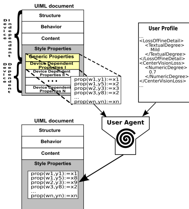
FIGURE 3: Applying a user profile to a high-level user interface description
