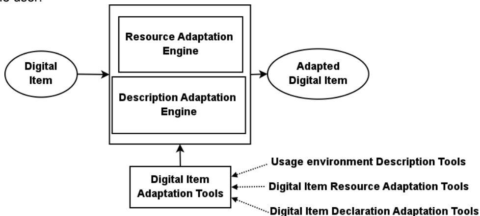
FIGURE 1: MPEG-21 Digital Item Adaptation overview from [13]
