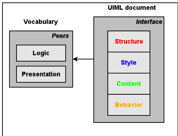
FIGURE 2: Structure of an UIML document
