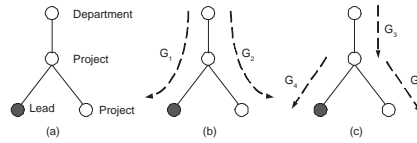
Fig. 3. Chain pattern tree for E_3 .
