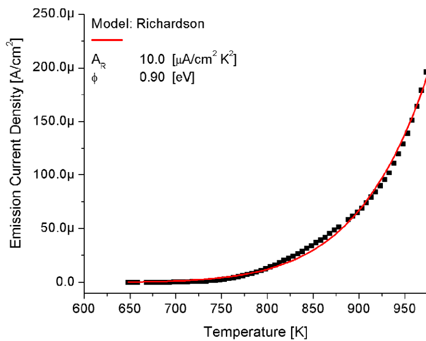
Figure 1. Thermionic electron emission data (squares) and fit to the Richardson relation (line) from phosphorus – doped polycrystalline diamond.
