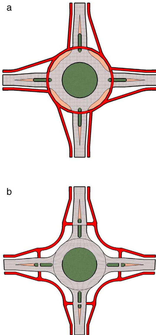
Fig. 3. Roundabouts with cycle path. a) Priority to bicyclists. b) No priority to bicyclists.
