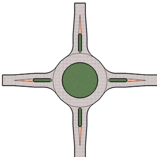
Fig. 1. Roundabout with mixed traffic.
