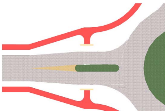
Fig. 4. Roundabout with grade-separated cycle path.
